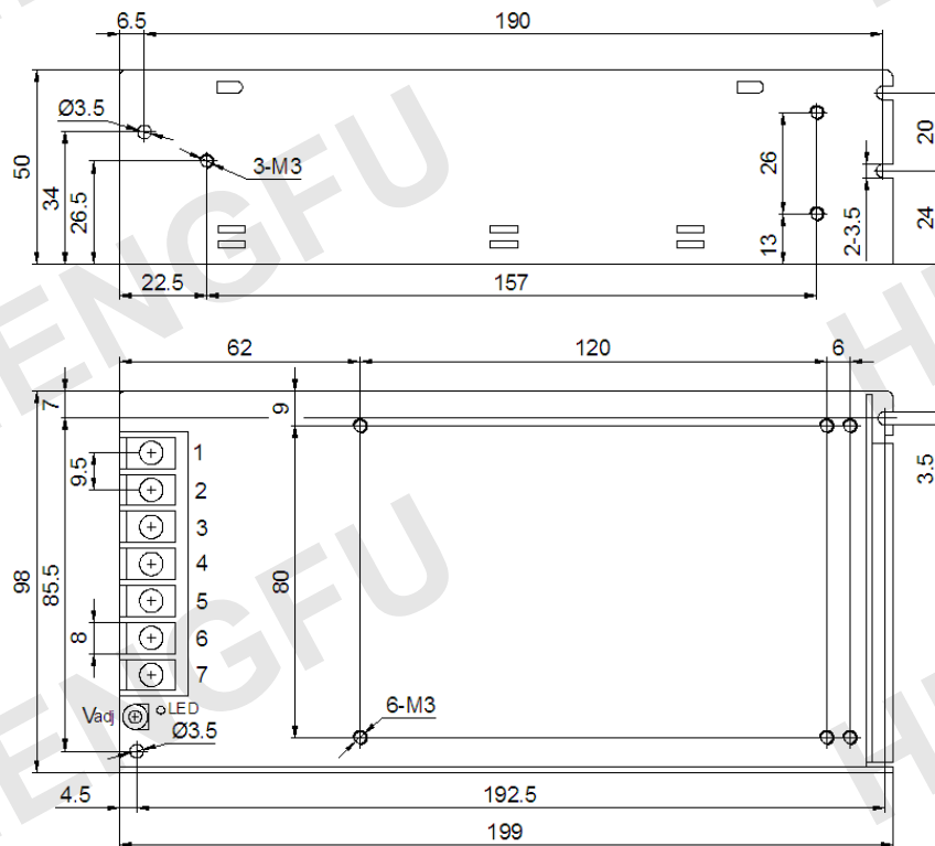
Terminal Pin No. Assignment 接线端子排布:
